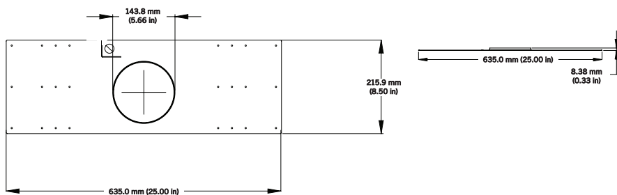
Pre-Construction Bracket (AC-CM3-PCB)
