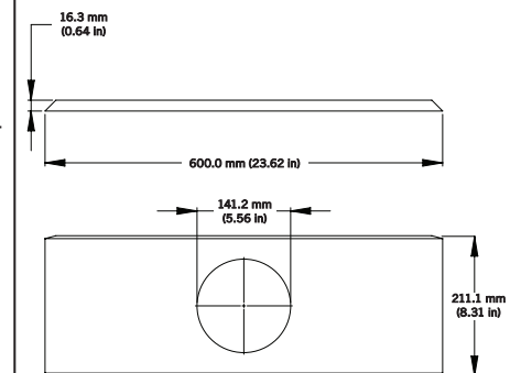
Tile Bridge
