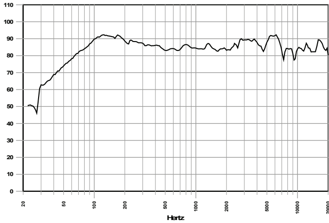
Frequency Response
