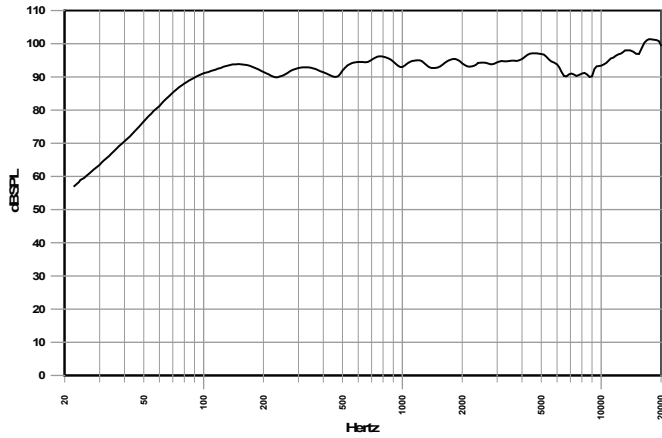
Frequency Response
