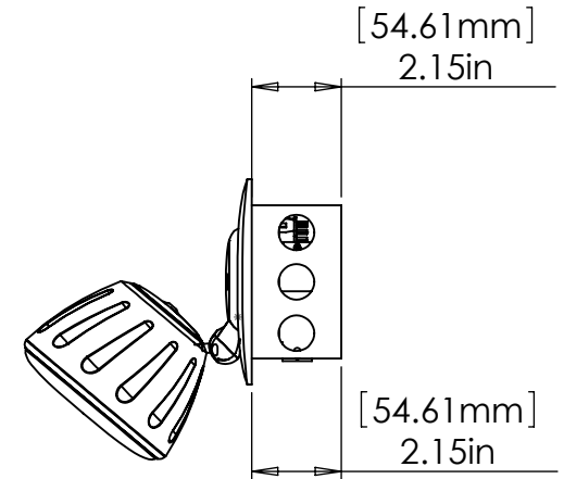
SM31-XFMR MOUNTED IN JUNCTION BOX
