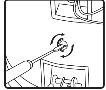
4. Set tap to proper setting. CM-EZ-8 is factory preset in the 70.7 Volt mode in the 20 Watt setting.
