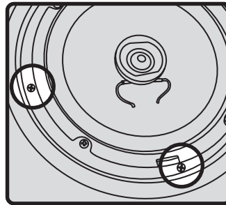
To Uninstall Speaker 1. Remove grille and locate brass release pins (x4).
