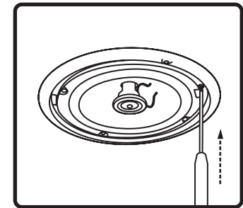
2. Using a screwdriver, push release pin up to release cam. Turn clockwise until threads engage to lock cam. Properly terminate signal wire in ceiling.
