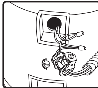
7. Thread tap & signal wires thru flexible conduit clamp. Connect wires with wire nuts. See tap settings on front page of this manual for proper settings.
