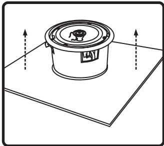
5. Lay tile bridge & tile on floor with tile facing up. Set speaker unit in hole and lift ceiling tile & tile bridge as a unit until speaker snaps into place.
